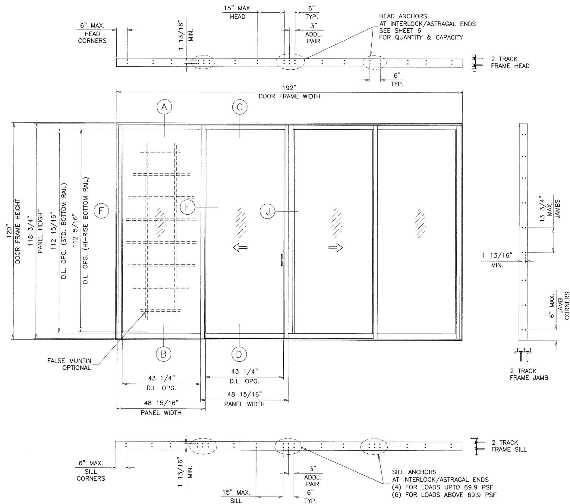
TYPICAL ELEVATION OX-XO
